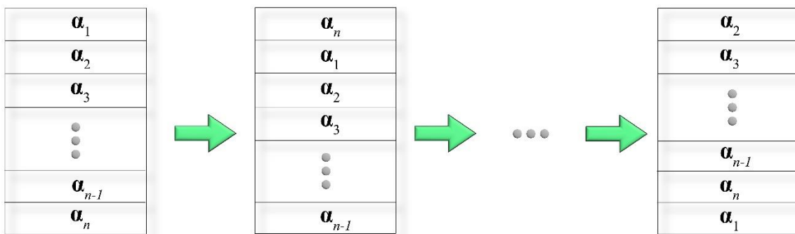
Figure 1. The variation of \alpha and its circular shift
