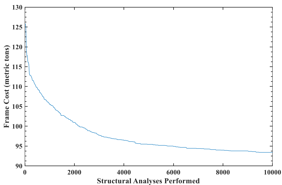
Figure 12. Convergence histories related to the best results of 5 \times 5 frame with fully moment connections
